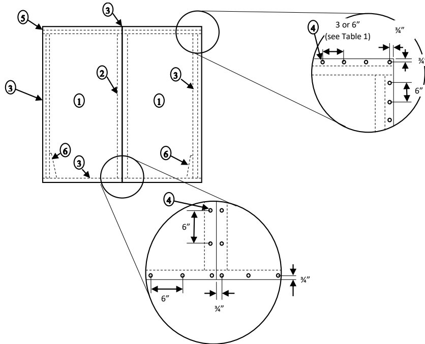
Figure 1: Typical Construction
